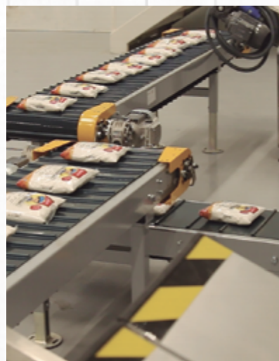
Details of the Tapioca's production line, Da Terrinha Alimentos – São Paulo, Brazil.
